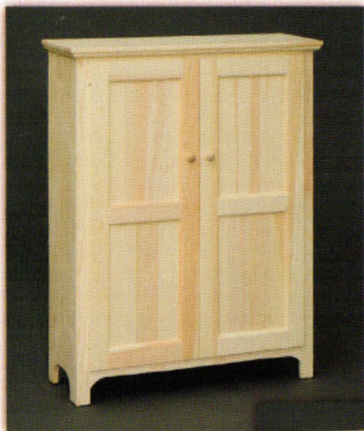
#8042 2 Door Pantry 38"w x 50"h x 13"d 3 Adjustable Shelves
