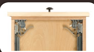
Undermount Soft-Close Drawer Slide (100-015US)
